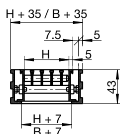
BGFG30MR H = 57 mm (32...82)
