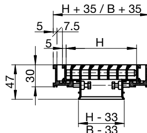
BGUG30MR H = 95, 145, 195 mm (95...495)
