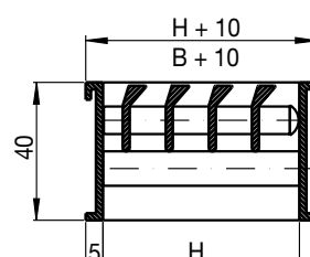
BGFS30 H = 57 mm (32...82)
